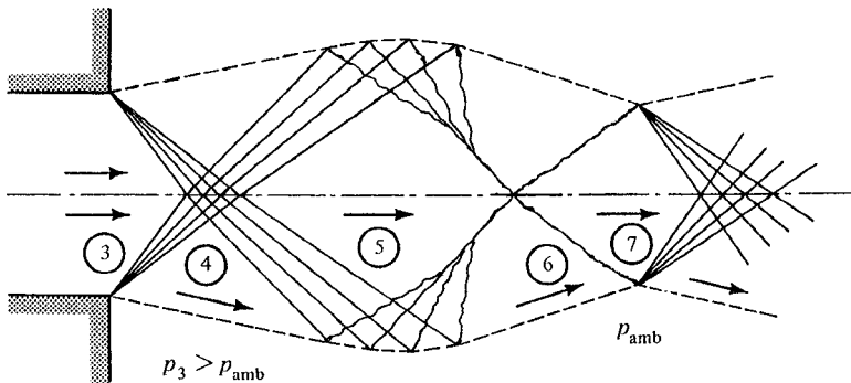
Figure 8.9 Underexpanded nozzle.
