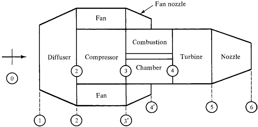
Figure 12.9 Basic parts of a turbofan engine.
