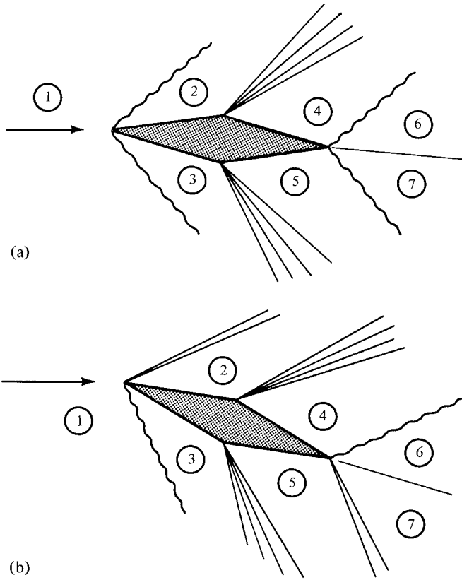
Figure 8.13 Double-wedge airfoil. (a) Low angle of attack. (b) High angle of attack.
