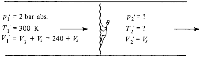
Figure 7.4 Moving shock transformed into stationary shock.
