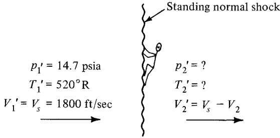
Figure 7.2 Moving shock transformed into stationary shock.
